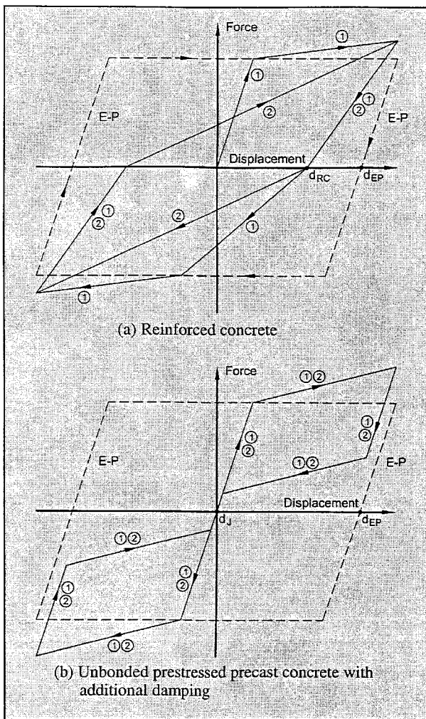
Fig. 1. Comparison of elasto-plastic and realistic hysteretic response.
