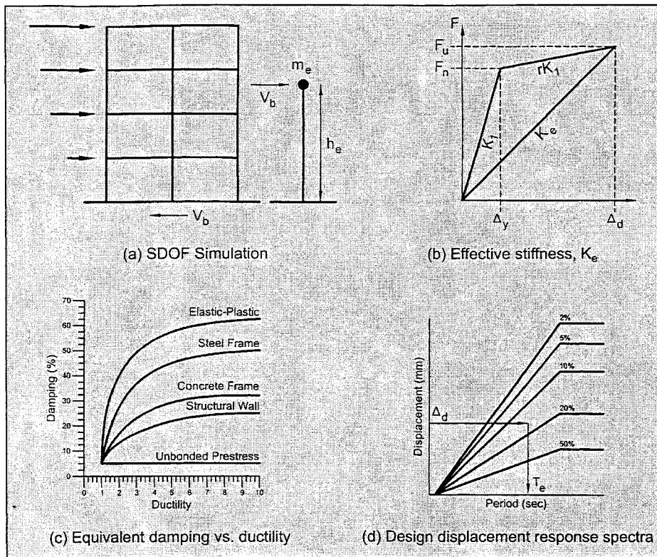
Fig. 3. Displacement based design fundamentals.
