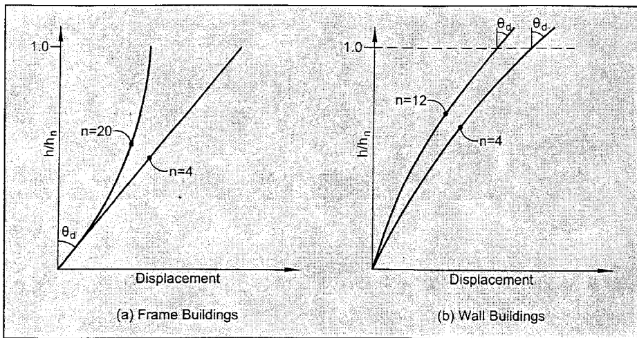
Fig. 4. Design displacement profiles for Direct Displacement-Based Design.
