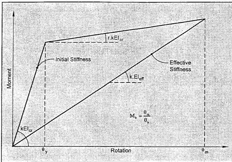
Fig. 5. Typical beam moment-rotation response.
