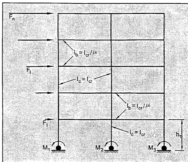
Fig. 6. Analysis of frame building.
