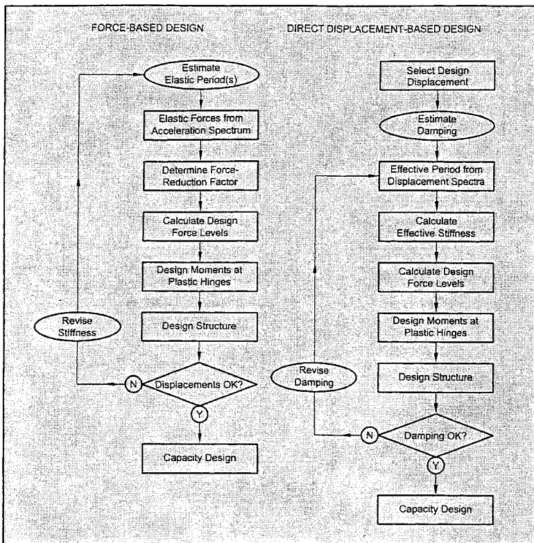
Fig. 2. Comparison of seismic design sequences.
